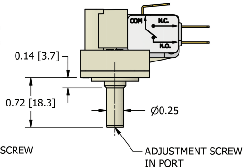
PORT STYLE -C- JOHN GUEST™ (QUICK DISCONNECT)
